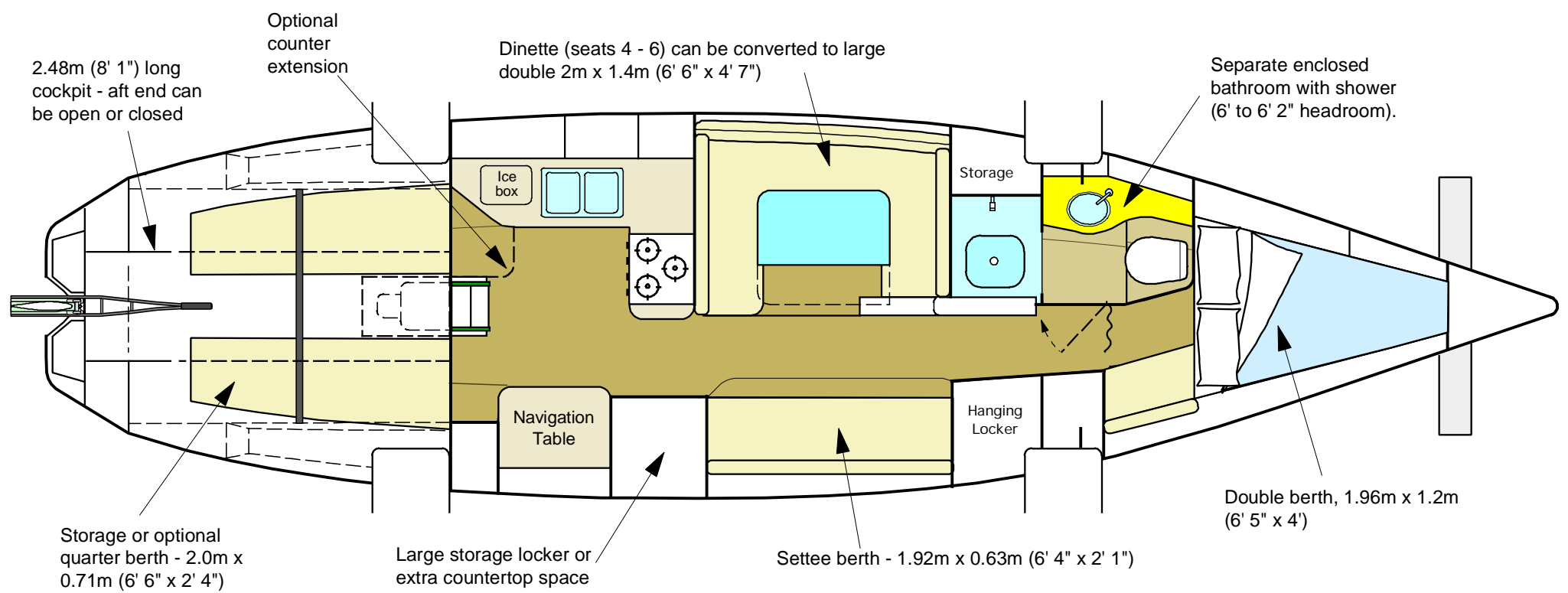
AFT COCKPIT CRUISING INTERIOR (With Longer Main Cabin and daggerboard)
