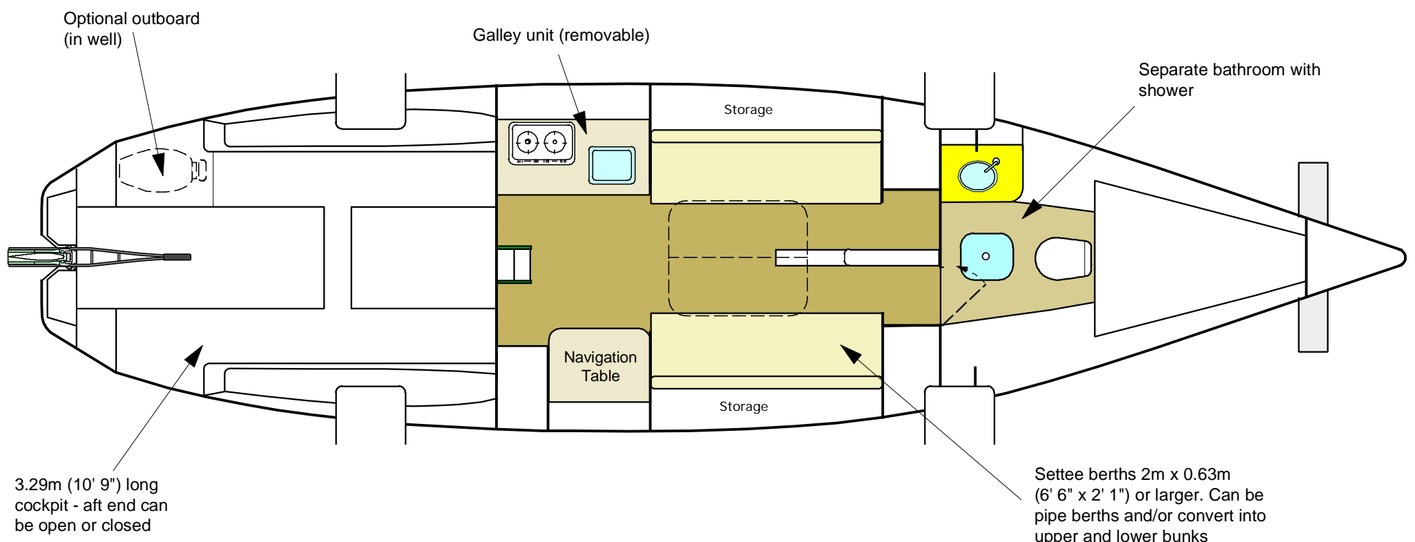
AFT COCKPIT F-39R/F-39ST INTERIOR (With Standard Main Cabin length and daggerboard)
