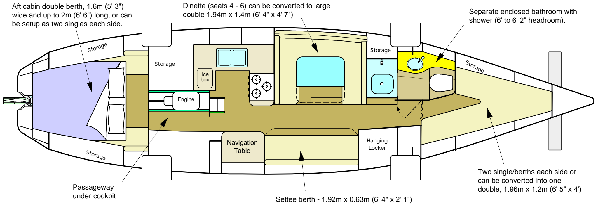
AFT CABIN FULL CRUISING INTERIOR (With Standard Main Cabin and optional 'kick-back' centerboard)
